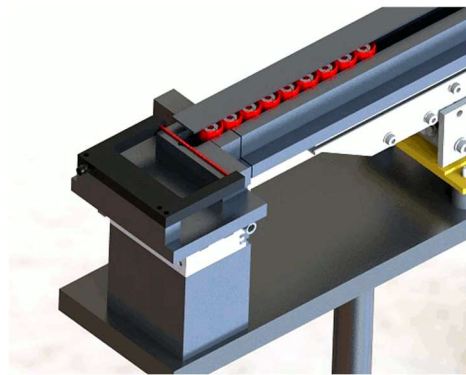
Pneumatic 2 position
