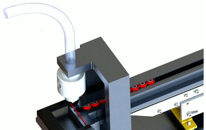
Blow Feed
